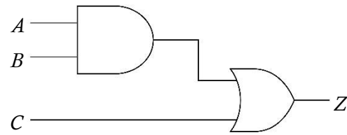
(b) Logic circuit based on Karnaugh map
